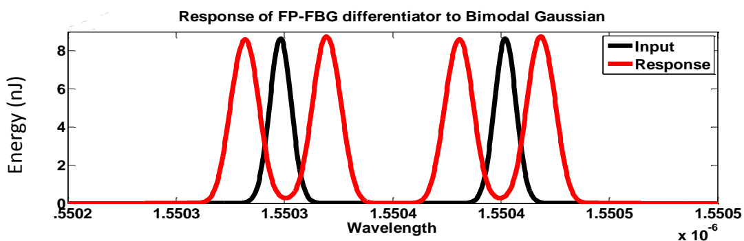
Fig. (4.5) Response of FP-FBG differentiator to a bi-modal Gaussian pulses
