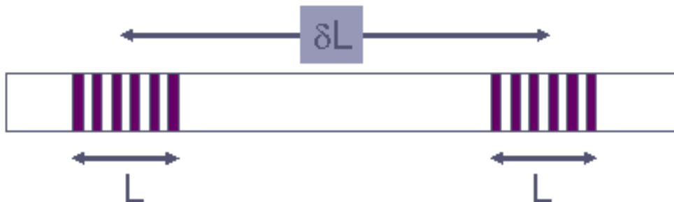
Fig. (2.14) Fabry-Perot filters using Fiber Bragg Gratings
