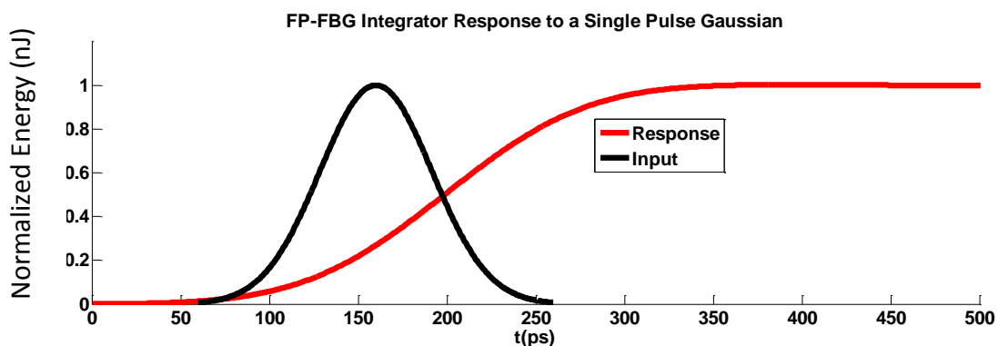
Fig. (3.11) FP-FBG integrator response to Gaussian pulse
