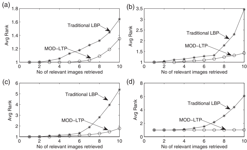
FIGURE 8. The average rank of retrieving 10 relevant images in different levels based on traditional LBP and iterated and weighted Moments of MOD-LTP with threshold 0.2 and window size 3. (a) L1, (b) L2, (c) L3, (d) L4.
