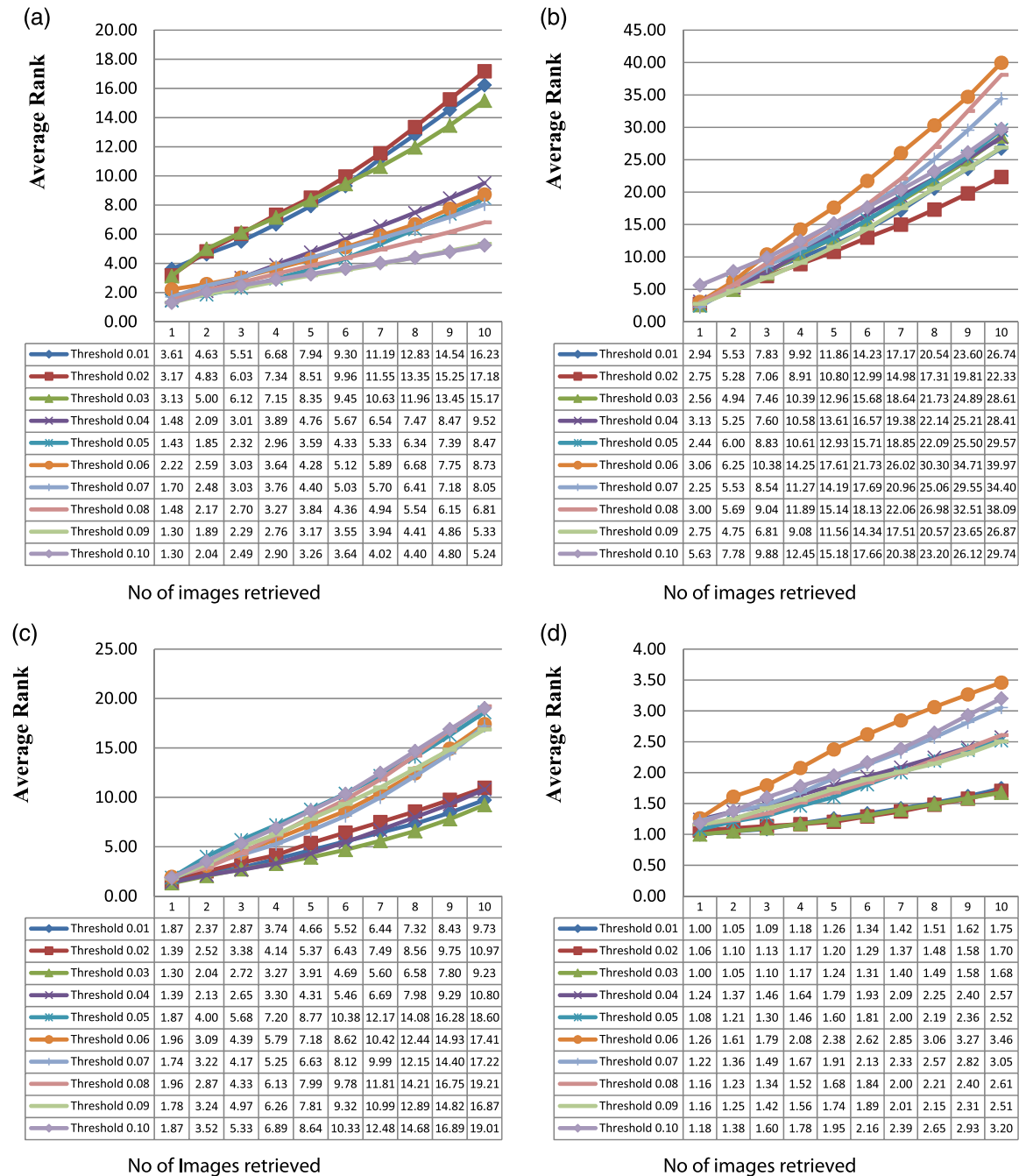
FIGURE 6. The average rank of set of queries with different threshold in each classes. (a) L1, (b) L2, (c) L3, (d) L4.
