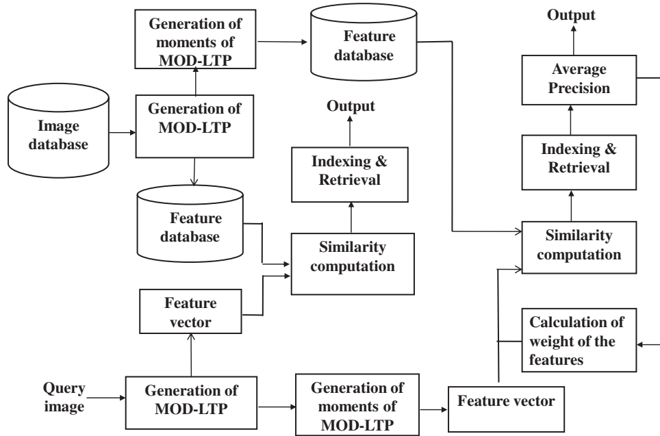
FIGURE 1. Block diagram of image retrieval scheme.
