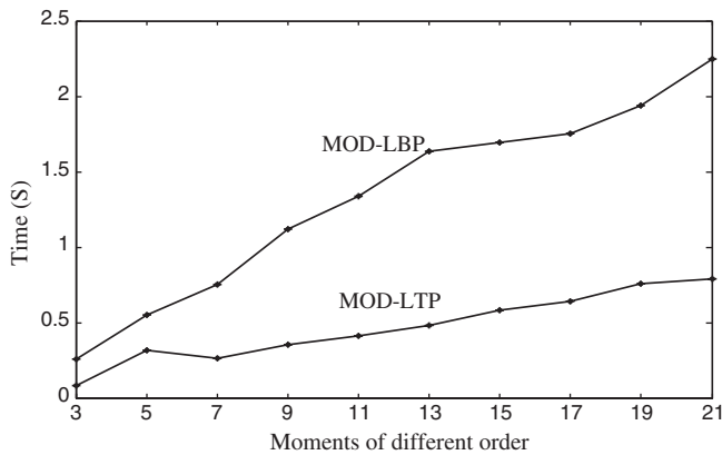
FIGURE 4. Time for calculating moments of different order.
