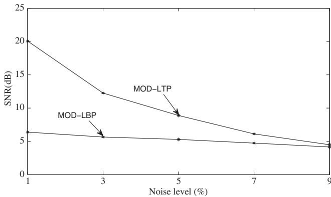
FIGURE 9. The SNR vs. noise level of MOD-LBP and MOD-LTP.
