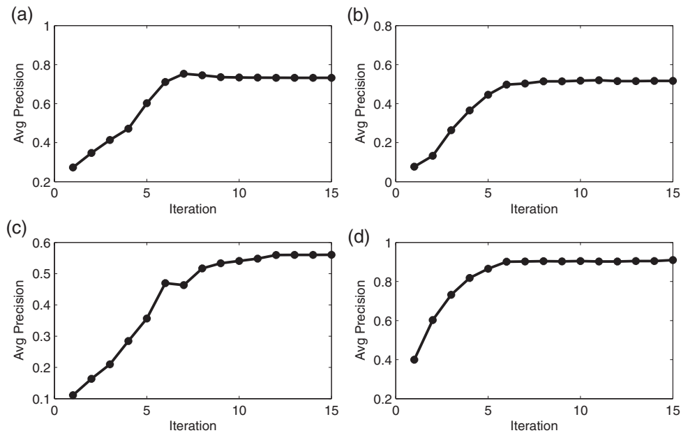
FIGURE 5. Average precision vs. iteration for (a) L1, (b) L2, (c) L3, (d) L4.
