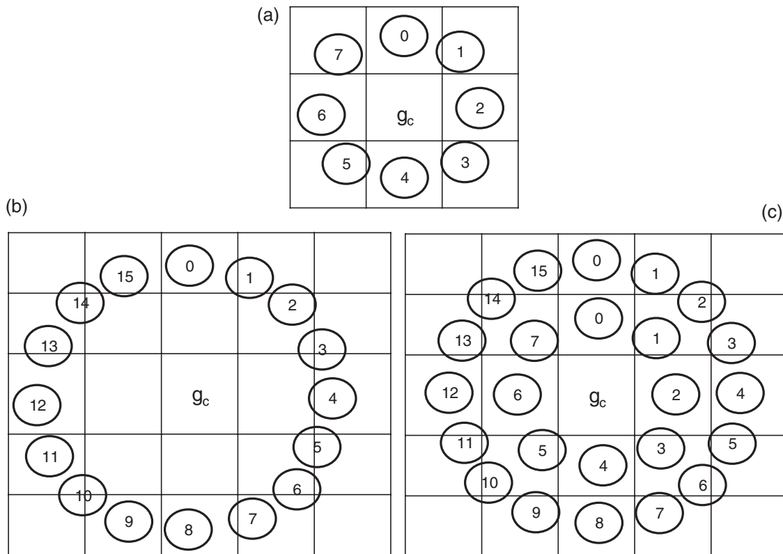
FIGURE 2. Pixel numbering of neighborhood pixels (a) for LBP and MOD-LTP computation with window size 3 (b) for LBP computation with window size 5 (c) for MOD-LTP computation with window size 5.
