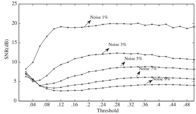
FIGURE 10. SNR vs. threshold of MOD-LTP over various noise levels.
