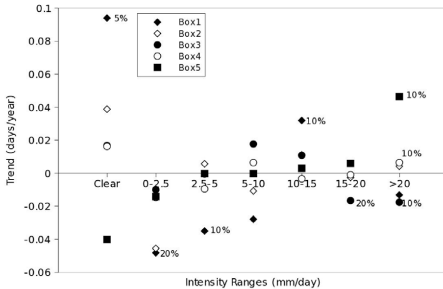
Fig. 5. Long term trends of number of rainy days in different intensity classes for all the five grid boxes. The significant levels corresponding to the values are given in the figure
