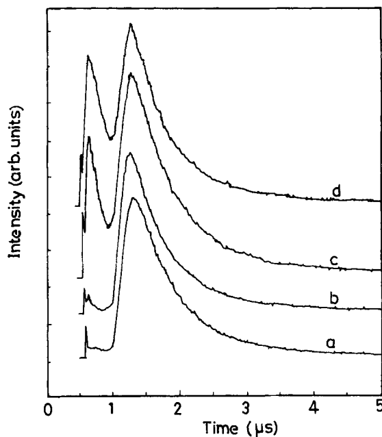
Figure 1. Intensity variation with time for 516.5 nm spectral emission from C_2 observed at 5 mm away from the target for laser fluences (a) 12.7 \text{ J cm}^{-2} (b) 26.7 \text{ J cm}^{-2} , (c) 28 \text{ J cm}^{-2} and (d) 29.3 \text{ J cm}^{-2} .
