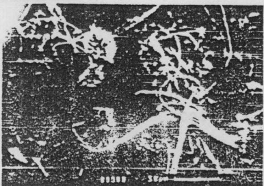
FIGURE 2e SEM photomicrograph of tear fracture surface of mix E. (Fibers in the longitudinal direction)
