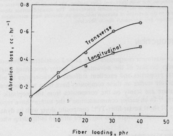
FIGURE 3 Variation of abrasion loss with fiber loading in the longitudinal and transverse directions.
