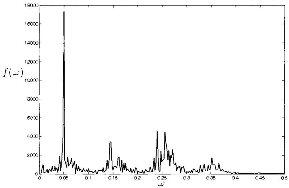
Figure 5.3: The power spectrum of the time series for the parameter values \Omega = 1.0 , \beta = 0.1 , a = 6.25 , \alpha = 80.0 and \omega = 0.3 .
