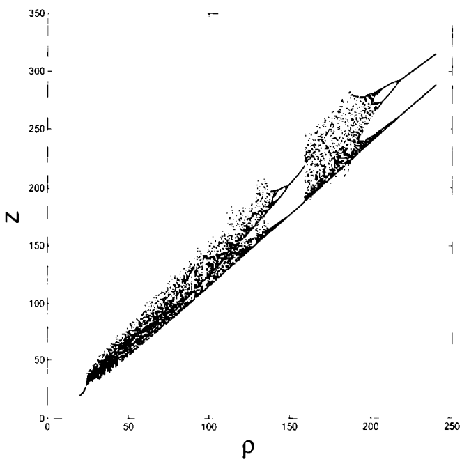
Figure 1.1: The bifurcation diagram of a Lorenz system.
