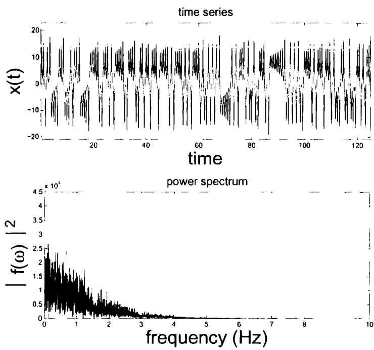
Figure 1.8: The time series and power spectrum of a chaotic Lorenz system.
