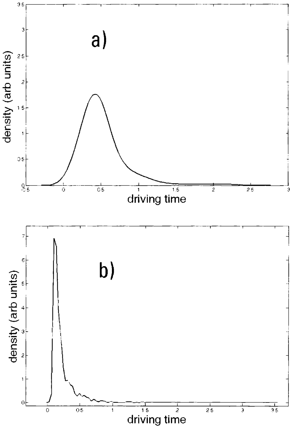
Figure 4.12: The density distributions of the driving times: a) deterministic driving b) stochastic driving
