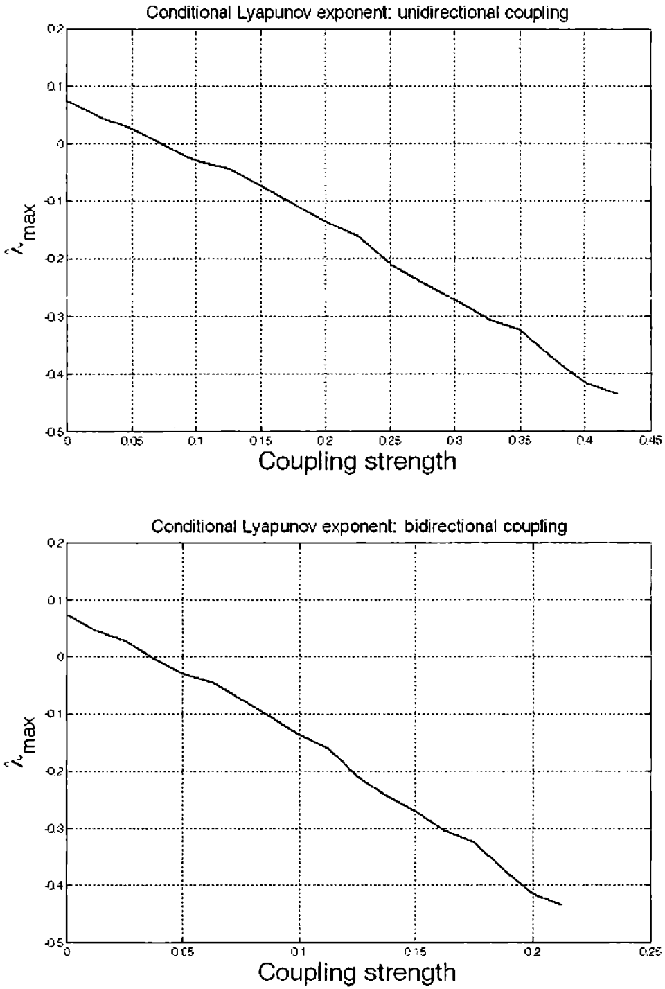
Figure 5.10: Variation of the maximal Conditional Lyapunov exponent with increase in coupling strength.
