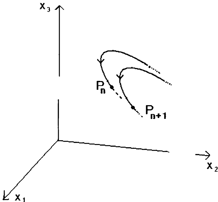
Figure 1.6: The schematic diagram of a Poincaré section.
