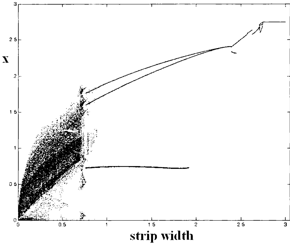
Figure 1.6: Bifurcation diagram obtained by varying the strip width s . Chaotic behavior disappears as the width of the strip is ( \Omega = 1.0 , \gamma = 0.1 , \omega = 0.3 and a = 2.5 ).
