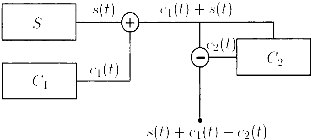
Figure 1.13: Schematic diagram of a secure communication scheme.
