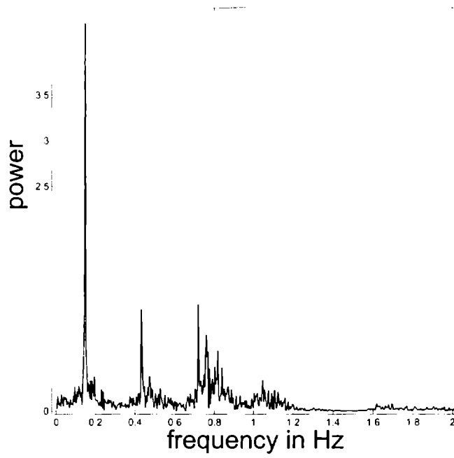
Figure 4.5: Power spectrum of the time series x(t) ( \Omega = 1.0 , \gamma = 0.1 , \omega = 0.3 , s = 0.1 and a = 2.5 ).
