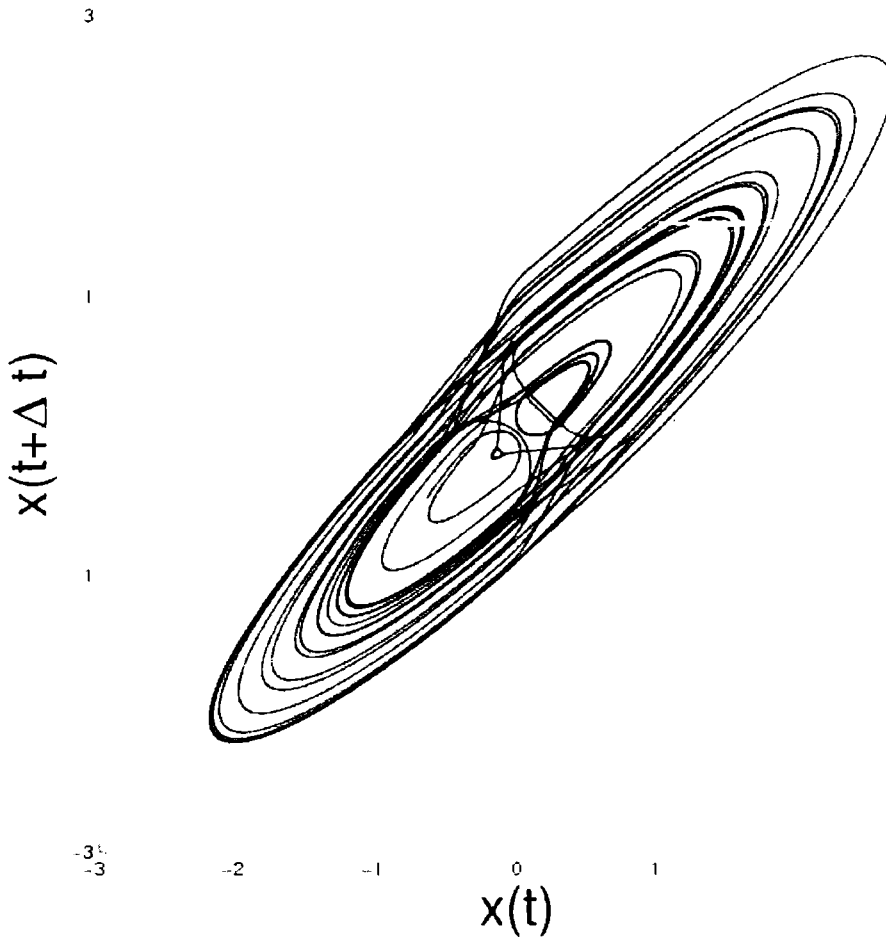
Figure 1.10: The reconstructed attractor resulting from random driving ( \Omega = 1.0 , \gamma = 0.1 , s = 0.1 , a = 2.5 and \Delta t = 1.1 ).
