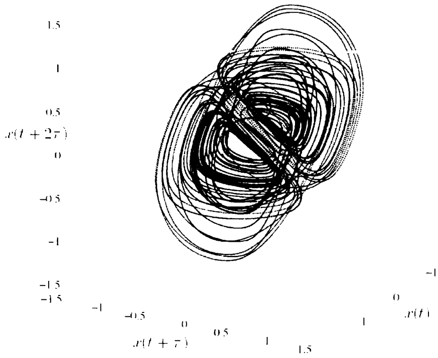
Figure 5.1: The delay reconstructed phase space of the oscillator.
