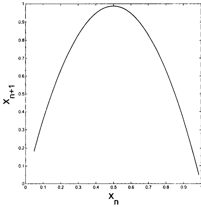
Figure 1.2: The return map of a logistic map.
