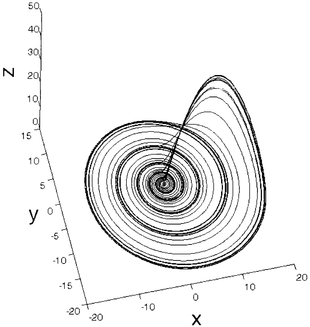
Figure 2.3: The phase space of the Rossler oscillator.
