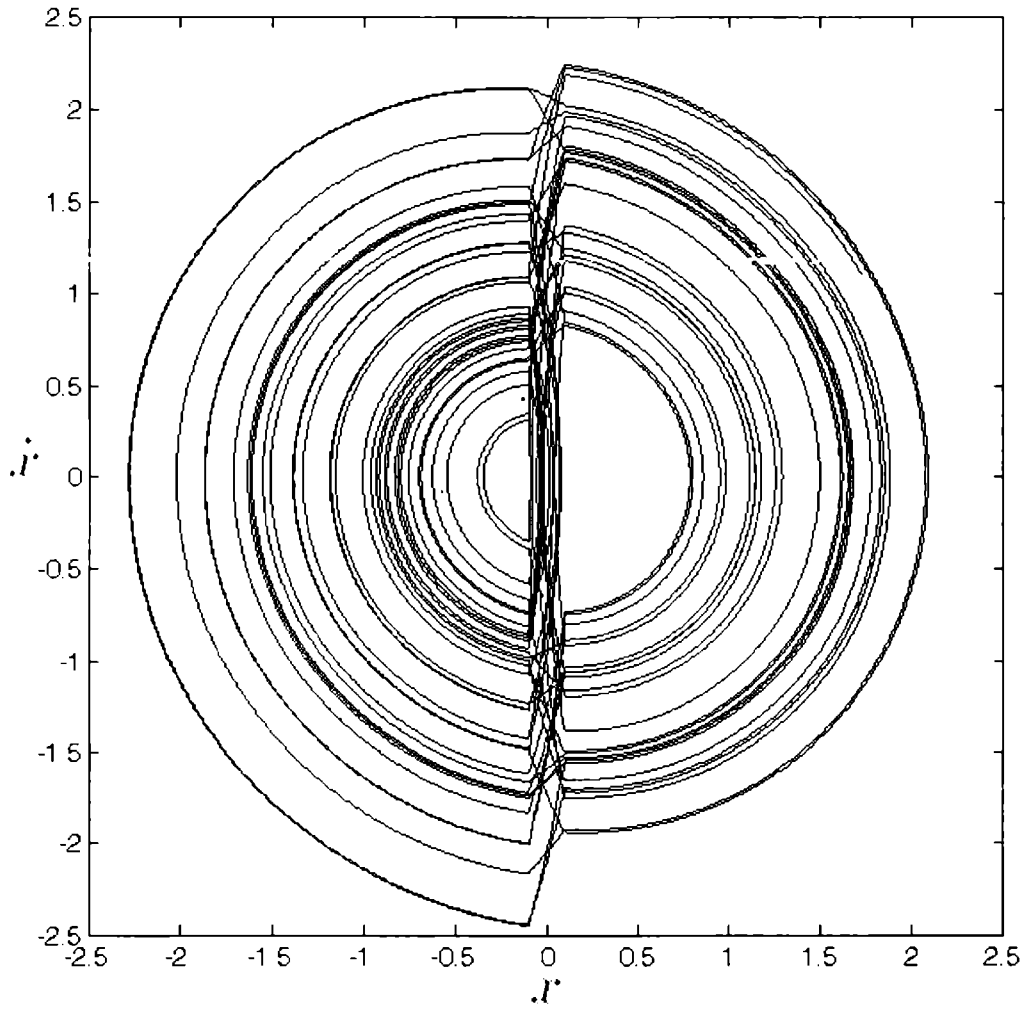
Figure 4.9: The position-momentum space of the oscillator under random driving. ( \Omega = 1.0 , \gamma = 0.1 , s = 0.1 , a = 2.5 and \Delta t = 1.1 ).
