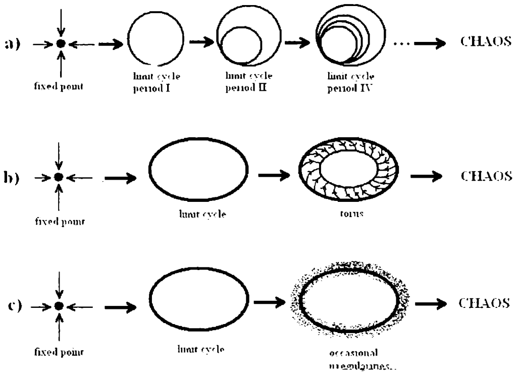
Figure 1.10: Routes to chaos: (a) period doubling route (b) quasiperiodicity route (c) intermittency route
