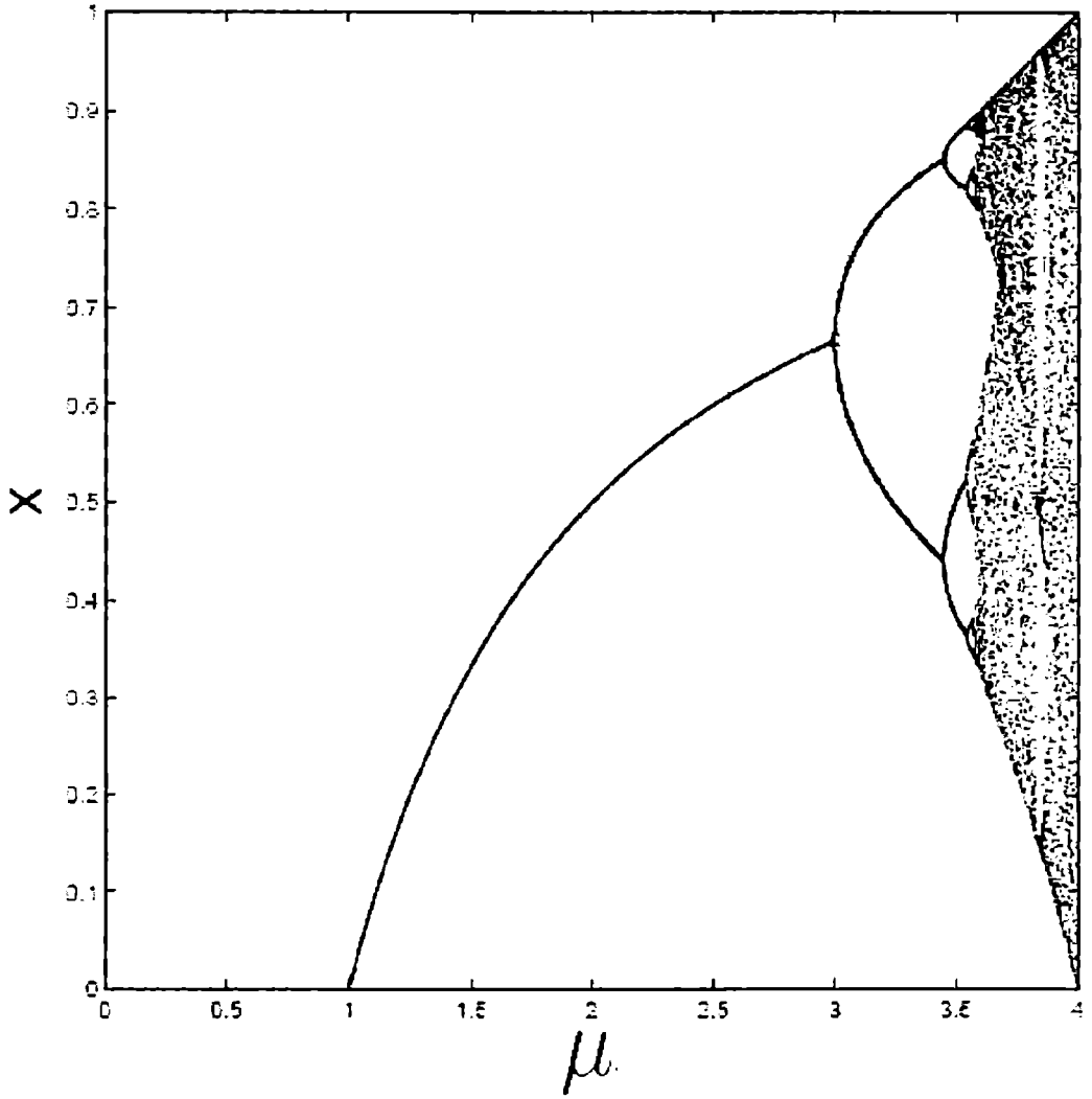
Figure 1.1: The bifurcation diagram of a logistic map.
